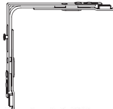
Corner transmission 1 ML Spindle 7 mm Screws M 5 x 35 Catch pin
