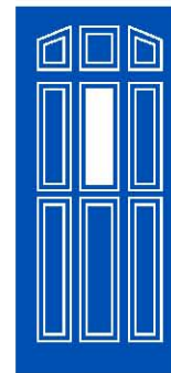
7K Centre Panel for 9-panel door Cut out: 216 x 496mm Glass: 190 x 469mm
