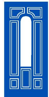
9M Centre Panel for 8-panel door Cut out: 275 x 1069mm Glass: 248 x 1042mm
