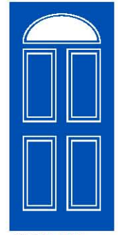
9W Half Moon Cut out: R292 X 279mm Glass: R279 x 254mm
